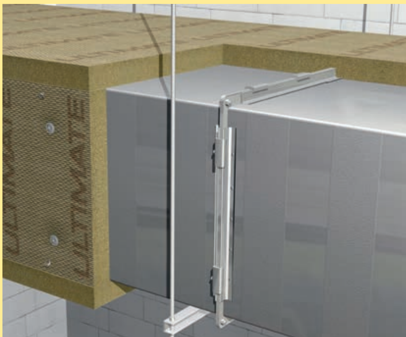
U PROTECT WIRED MAT 4.0
